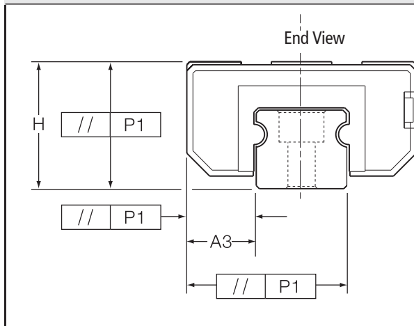
Figure 1 - Dimensions H and A3
