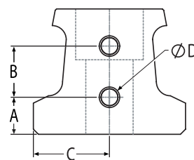
Rail End Machine Detail
