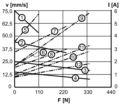
Speed and Current vs. Load 12 and 24 Vdc
