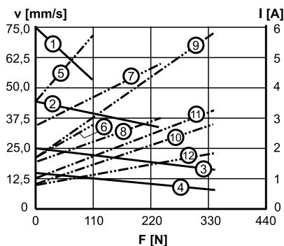
Speed and Current vs. Load 12 and 24 Vdc
